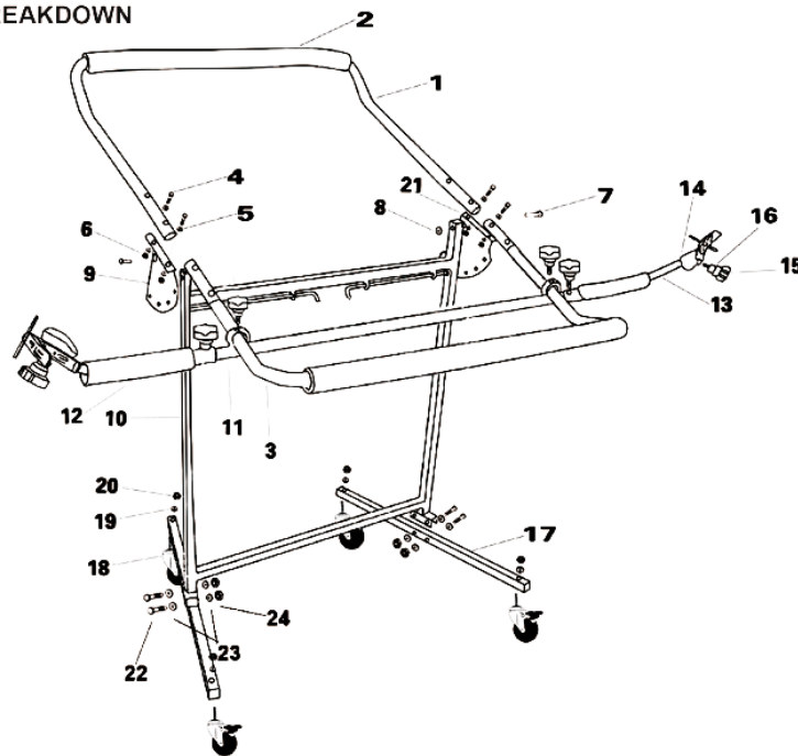
PARTS BREAKDOWN
